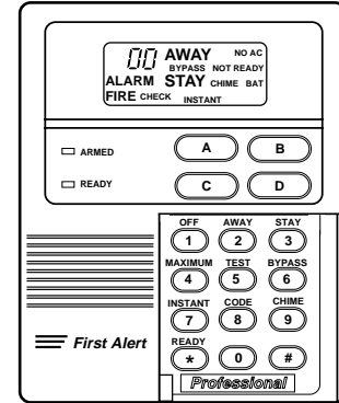
FA250KP FIXED-WORD KEYPAD (STYLE B DISPLAY)
